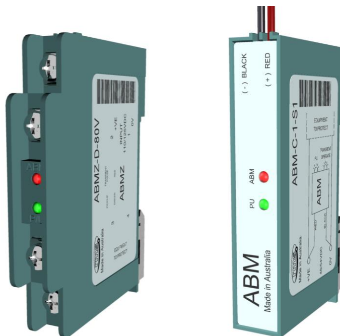
ABM Active Burden Modules (‘Screw terminal’ and ‘Flying lead’ versions depicted)
