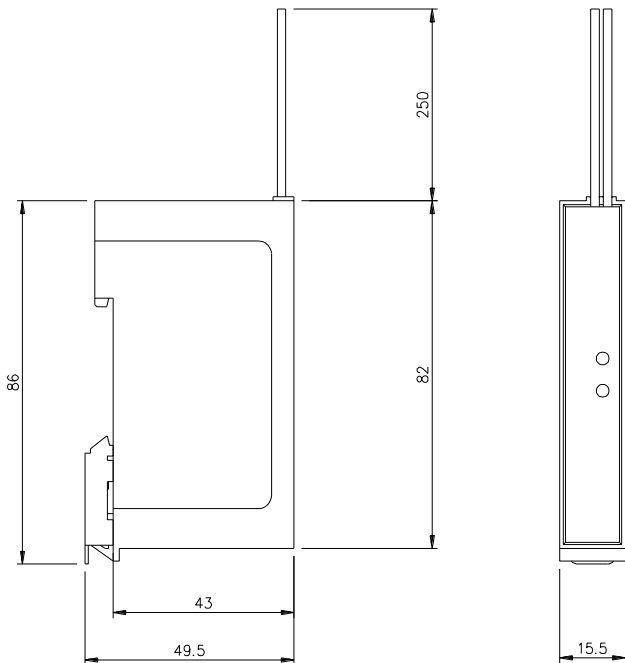
Figure 12: ABM 'Flying lead' version dimensional details
