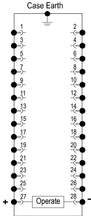
Case terminations (REAR VIEW)
