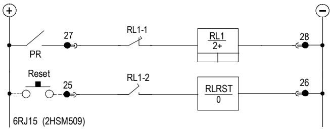
Relay circuit diagram
