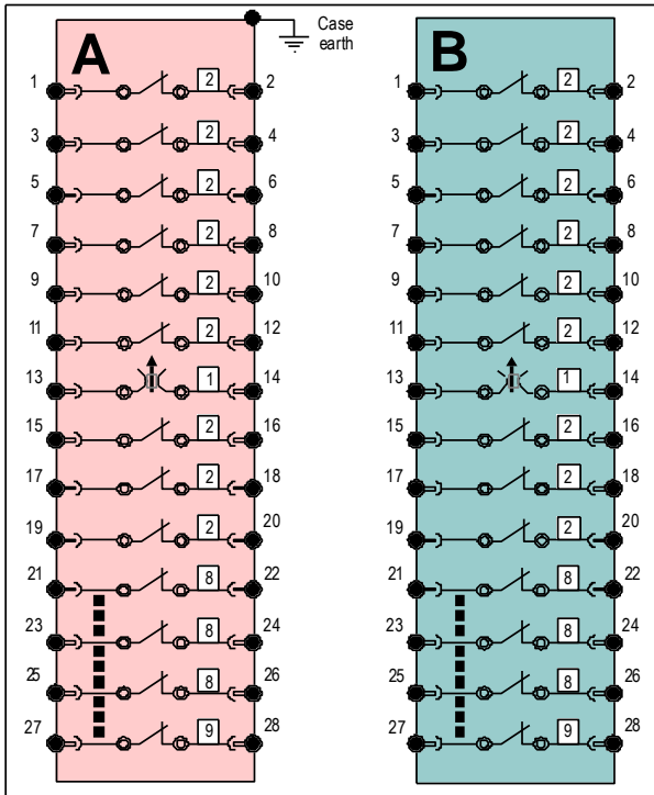
Figure 9: Viewed from rear terminal side Full order code: 4M402-S- 2 2 2 2 2 2 2 2 2 2 2 8 8 9 Short code: 4M402-06
