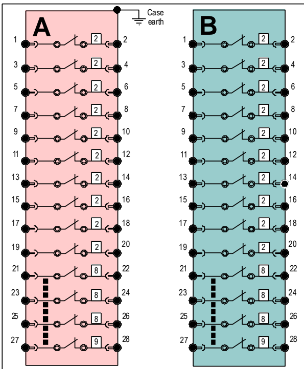
Figure 10: Viewed from rear terminal side Full order code: 4M402-S- 2 2 2 2 2 2 2 2 2 2 2 8 8 8 9 Short code: 4M402-07
