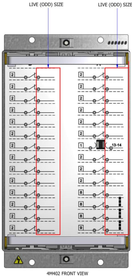
Figure 5: Position of Live Side terminals on 4M402-S Order Code versions
